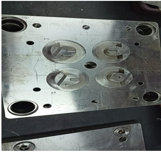
Product: Injection Mould (4 Cavities), Customer: M/s ALIMCO
